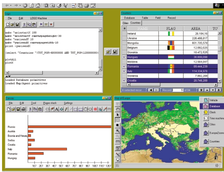
Figure 2. An E-Slate geography lesson using logo (scripting), database, canvas, and map components.
